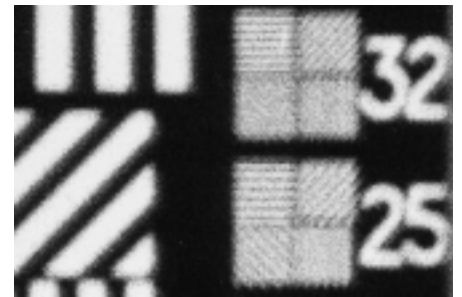
Film displaced only 0.3mm ( 1/80'' ) from the optimum image plane (at full aperture).
